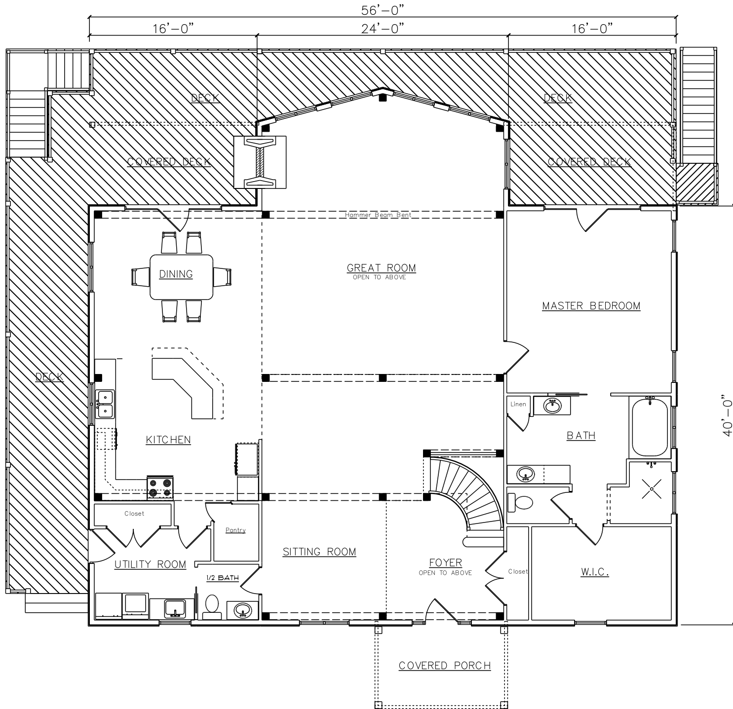
MAIN FLOOR LAYOUT
