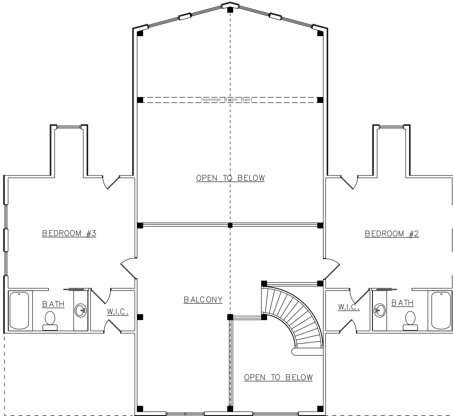
2ND FLOOR LAYOUT
