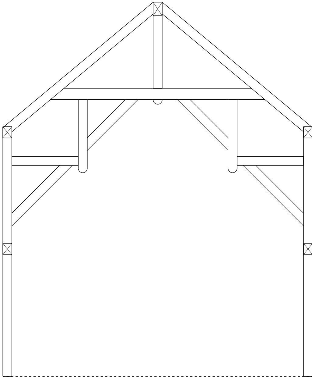
HAMMER BEAM DESIGN
