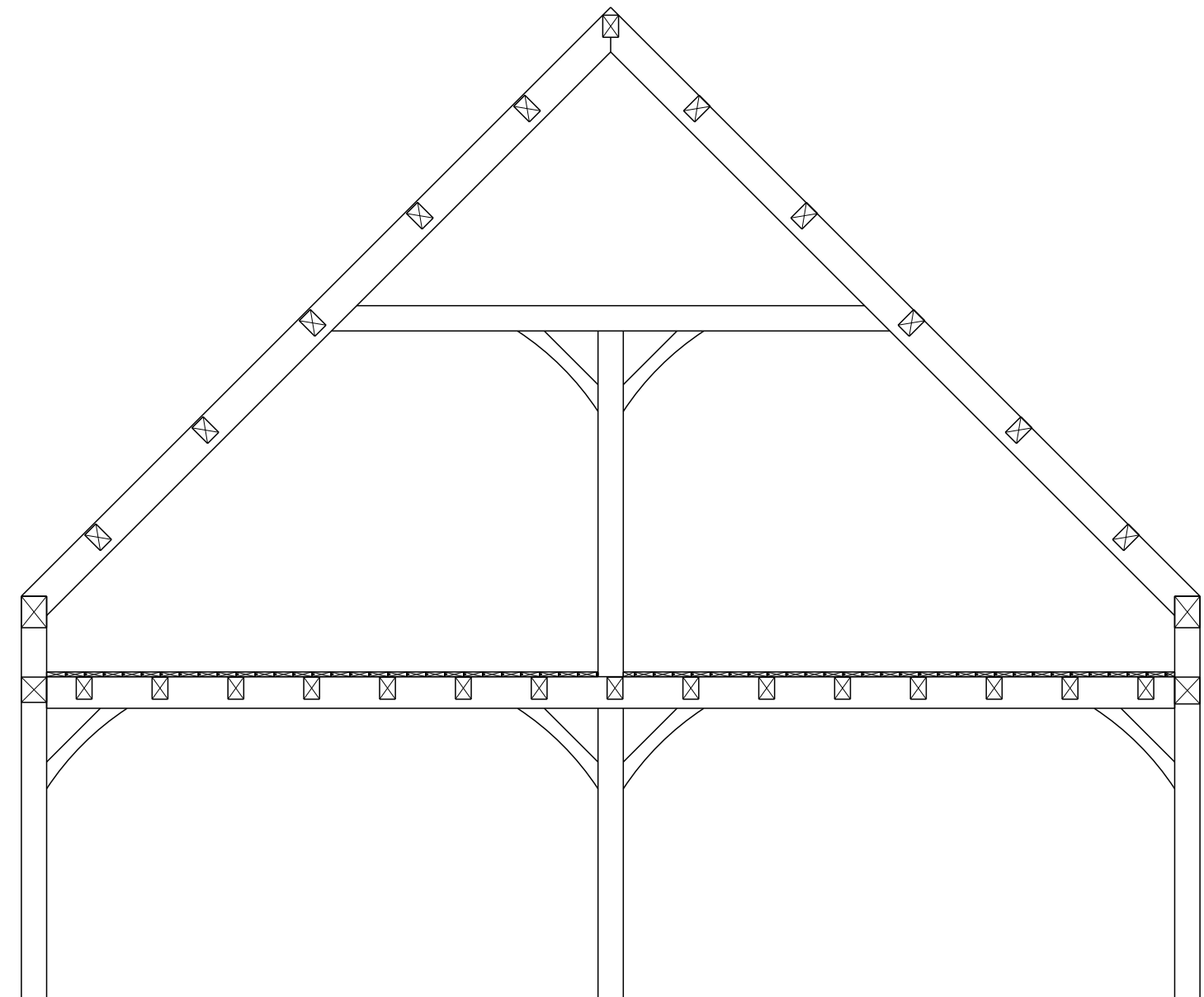
KING POST DESIGN
